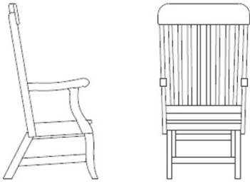
ROC01 Stable Base Rocker 28"d x 26"w x 45"h 27" arm ht 17" seat ht 35" rocking depth, 28" stable depth
